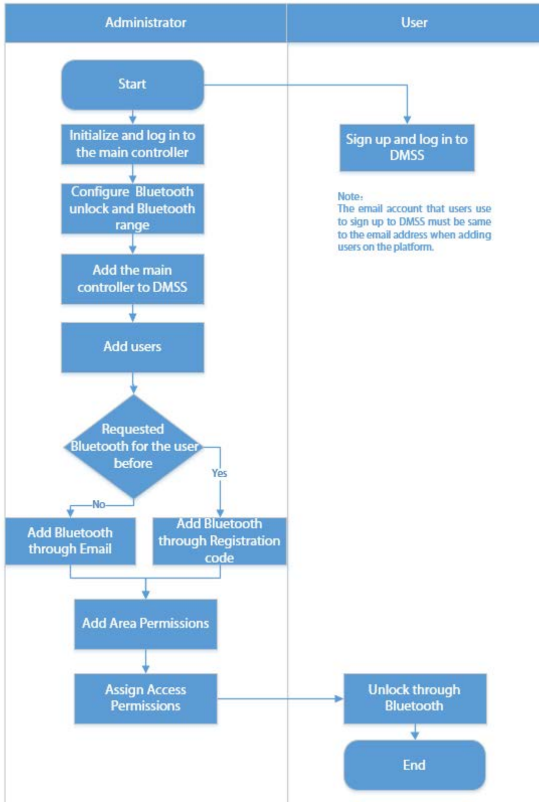
Figure 2-17 Flowchart of configuring Bluetooth unlock
