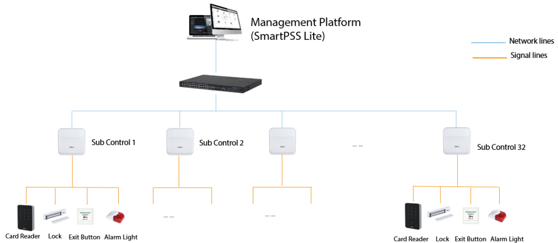
Figure 3-1 Networking Diagram
