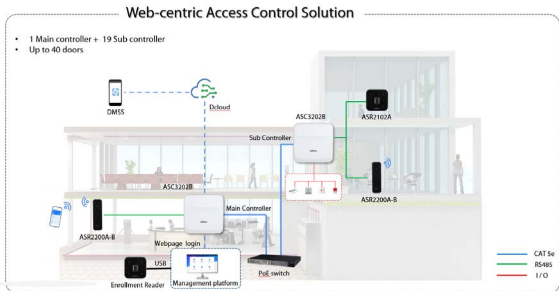
Figure 2-1 Networking diagram
