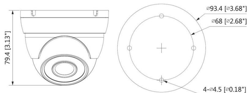
Figure 2-1 (mm [in])
