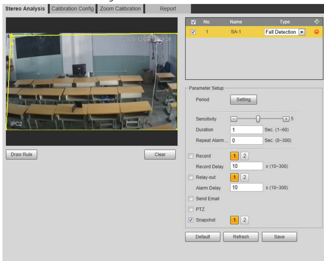
Figure 5-79 Fall detection
