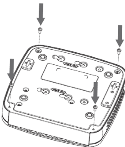
Figure 2-35 Fasten screws
