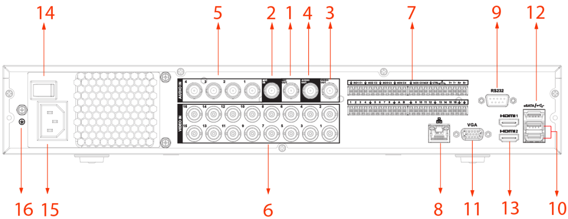
Figure 3-20 Rear panel (3)
