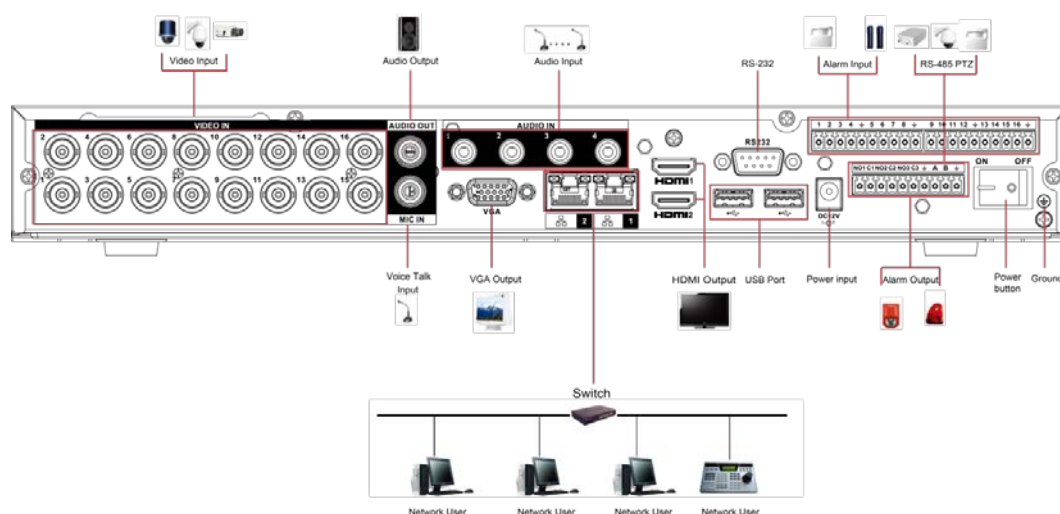
Figure 4-1 Connection diagram
